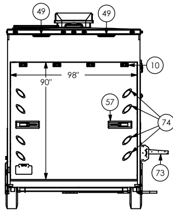
EXTERIOR REAR
