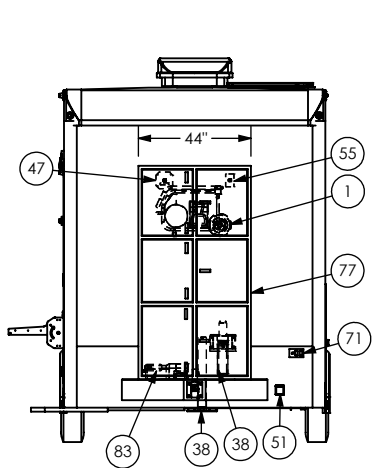
EXTERIOR FRONT
