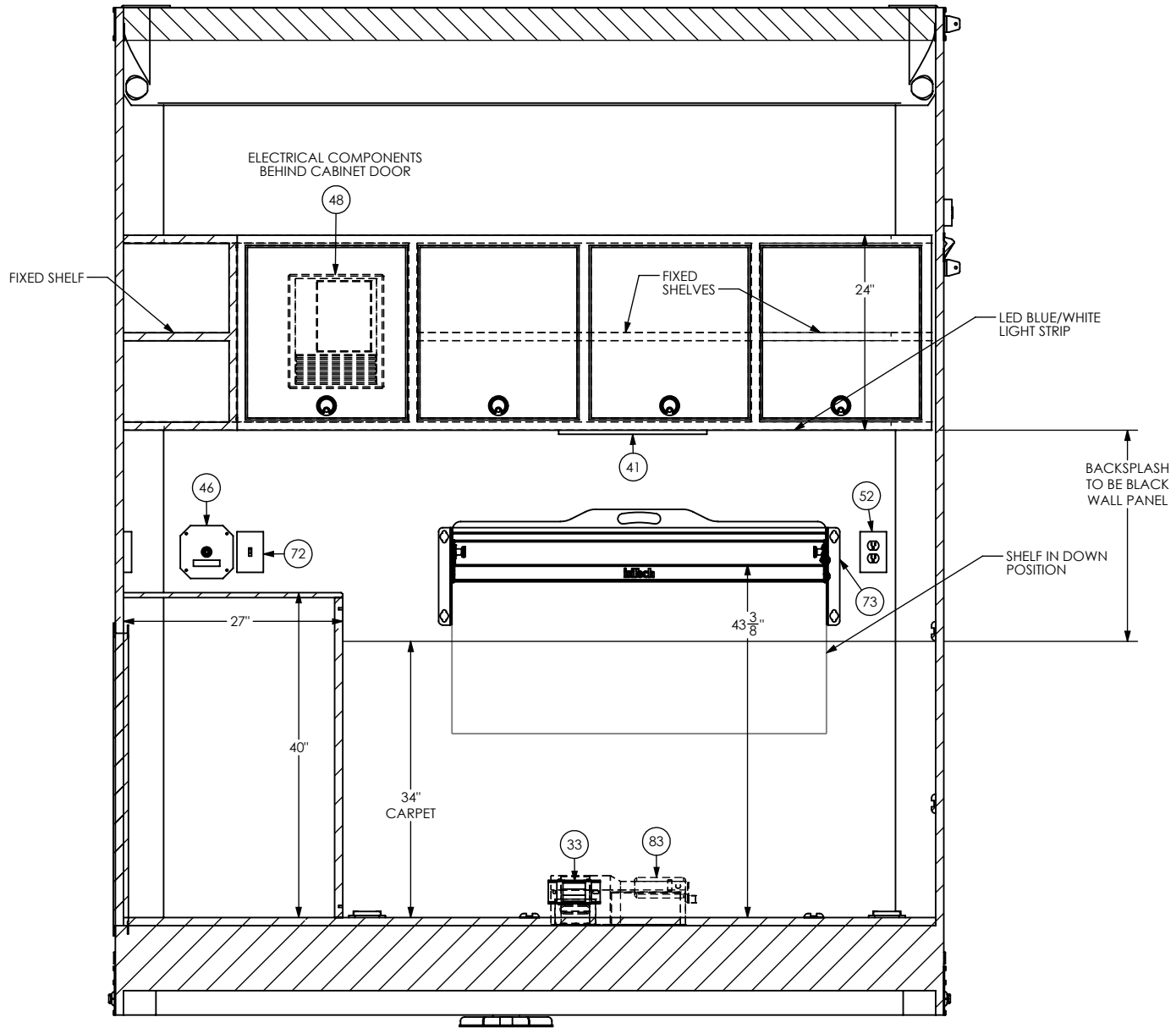
INTERIOR FRONT SECTION C-C
